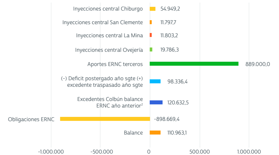
BALANCE ERNC (MWh)
